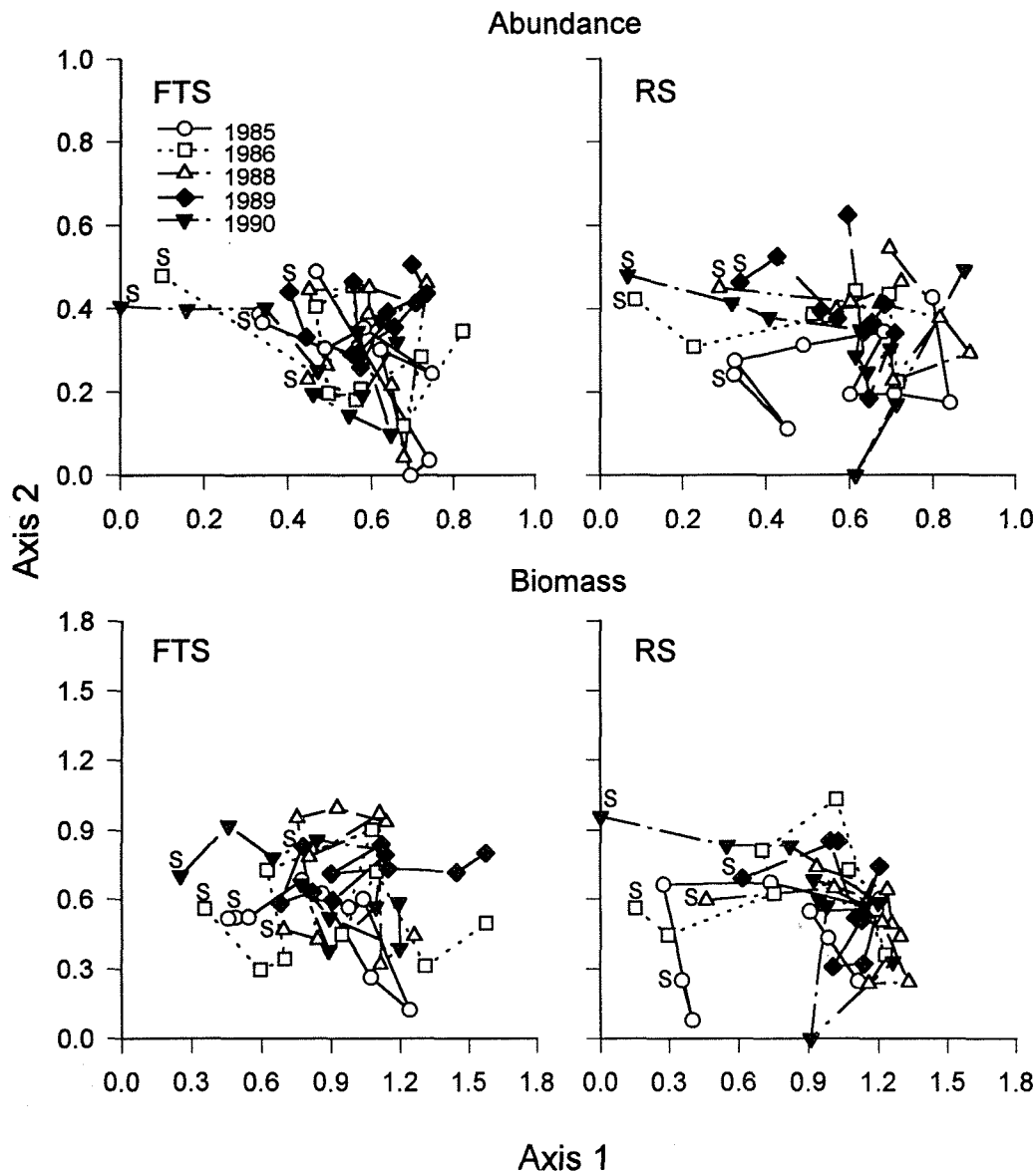
FIG. 8. Ordination plots of the first 2 axes from detrended correspondence analyses for the abundance (top) and biomass (bottom) of 11 macroinvertebrate taxa in the former treatment stream (FTS) and in the reference stream (RS) on each collection date. Open symbols represent drought years (1985, 1986, 1988) and closed symbols represent wet years (1989, 1990). The 1st collection date each year is denoted by S and subsequent collections are connected by the same line.
