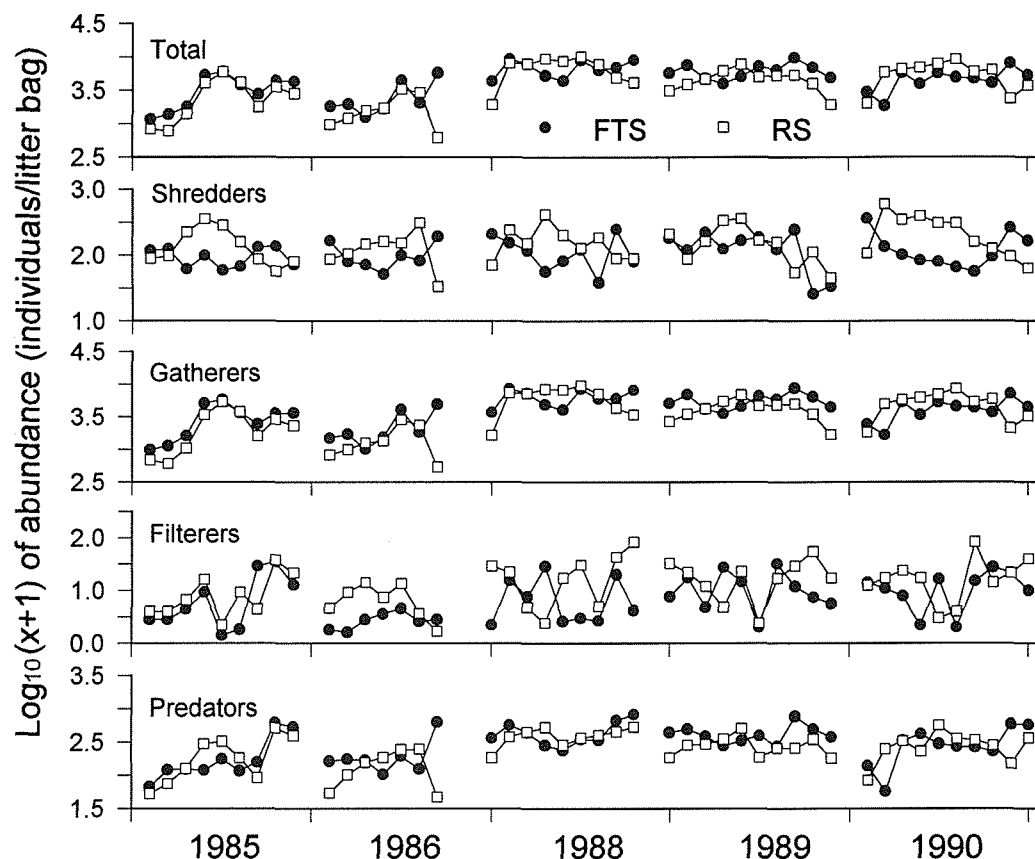
FIG. 3. \log_{10}(x + 1) -transformed mean abundance of total macroinvertebrates and each functional feeding group in the former treatment stream (FTS) and in the reference stream (RS) on each date of litter bag collection.
