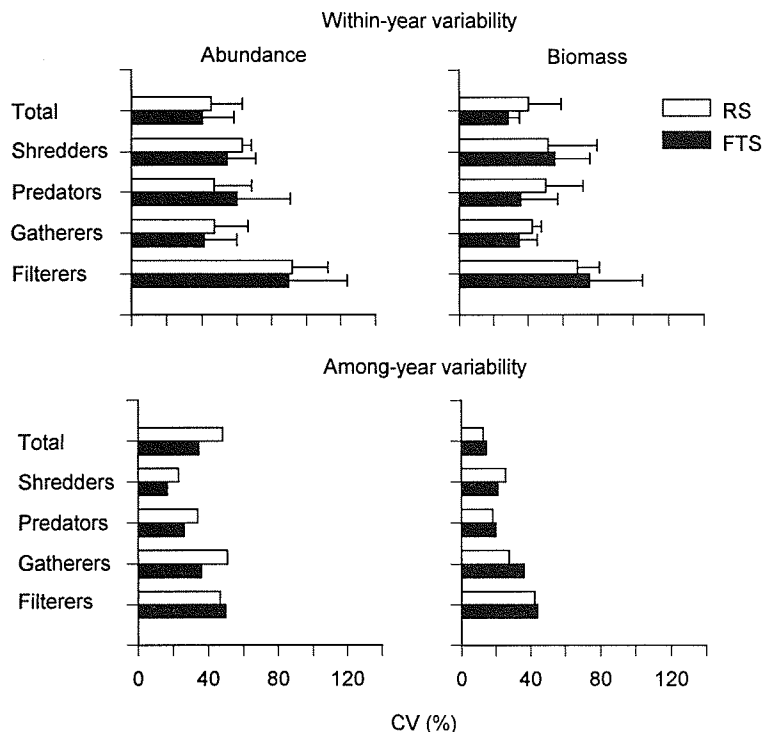
FIG. 5. Mean within- (top) and among-year (bottom) coefficients of variation (CV) for total macroinvertebrate and each functional feeding group abundance (left) and biomass (right) in the former treatment stream (FTS) and in the reference stream (RS). Error bars for within-year CVs represent +95% confidence intervals.
