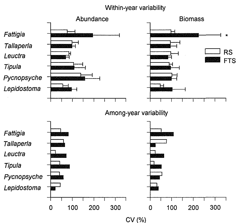
FIG. 6. Mean within- (top) and among-year (bottom) coefficients of variation (CV) for the dominant shredder taxa based on abundance (left) and biomass (right) in the former treatment stream (FTS) and in the reference stream (RS). Error bars for within-year CVs represent +95% confidence intervals. Asterisk indicates a significant difference between FTS and RS ( p < 0.05 ).
