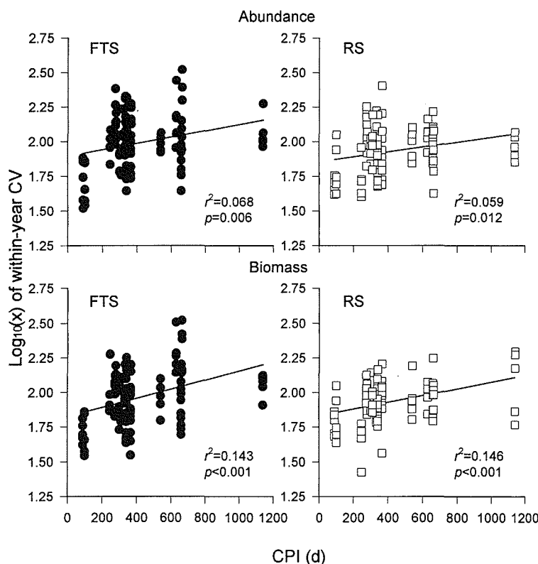
FIG. 7. Log 10 -transformed within-year coefficients of variation (CV) for 22 taxa based on abundance (top) and biomass (bottom) vs their respective cohort production interval (CPI) in the former treatment stream (FTS) and in the reference stream (RS). The lines are fitted regressions.
