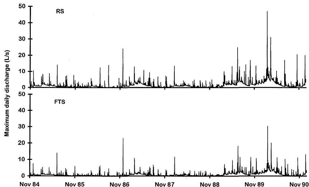
FIG. 1. Maximum daily discharge (L/s) in the reference stream (RS) and in the former treatment stream (FTS) during our study.
