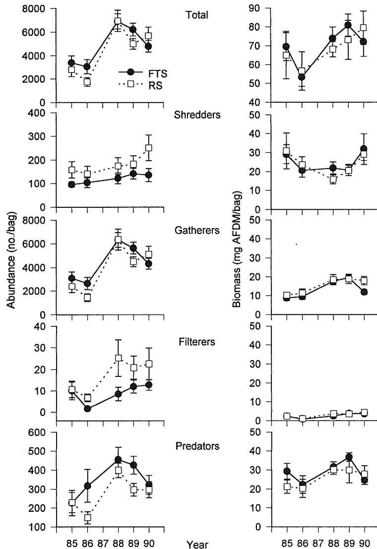
FIG. 2. Annual means ( \pm 1 SE) for abundance and biomass of each functional feeding group and total macroinvertebrates in the former treatment stream (FTS) and in the reference stream (RS) vs year. In some cases the error bars are hidden by symbols.
