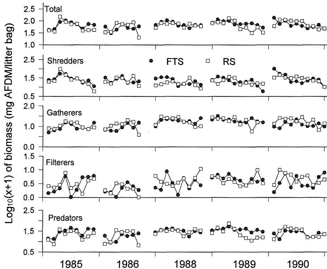
FIG. 4. \text{Log}_{10}(x+1) -transformed mean biomass of total macroinvertebrates and each functional feeding group in the former treatment stream (FTS) and in the reference stream (RS) on each date of litter bag collection.
